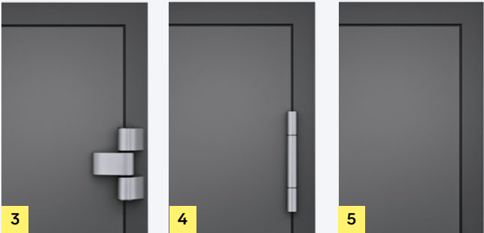
3| Screw-on hinge. 4| Roller hinge. 5| Concealed hinge.
